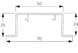
SG 2615 Recess profile
