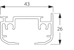
SG 2601 Profile
