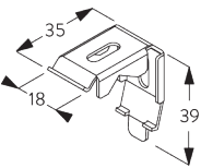
SG 2302 Bracket
