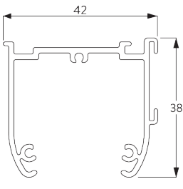
SG 2321 Profile
