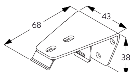
SG 2363 Bracket 68 mm
