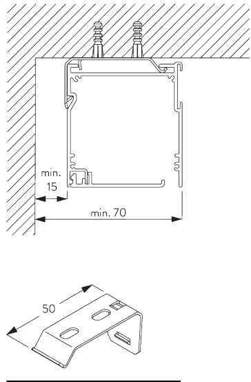
SG 2521 Bracket
