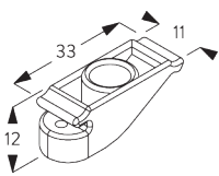
SG 2338 Side guide wire holder
