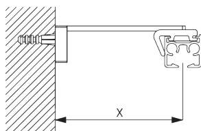
Square Smart Fix SG 11210 - SG 11215 and bracket SG 3826:
