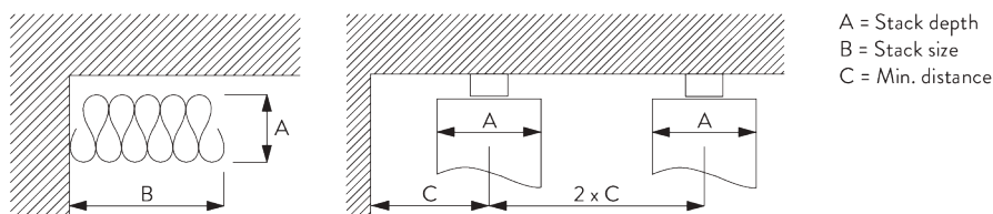
Wave stack depth - 2C glider cord (standard components)
