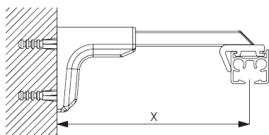
Universal Smart Fix SG 11154 - SG 11156 and bracket SG 3826:
