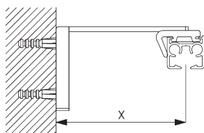
Smart Fix SG 11200 - SG 11205 and bracket SG 3826:
